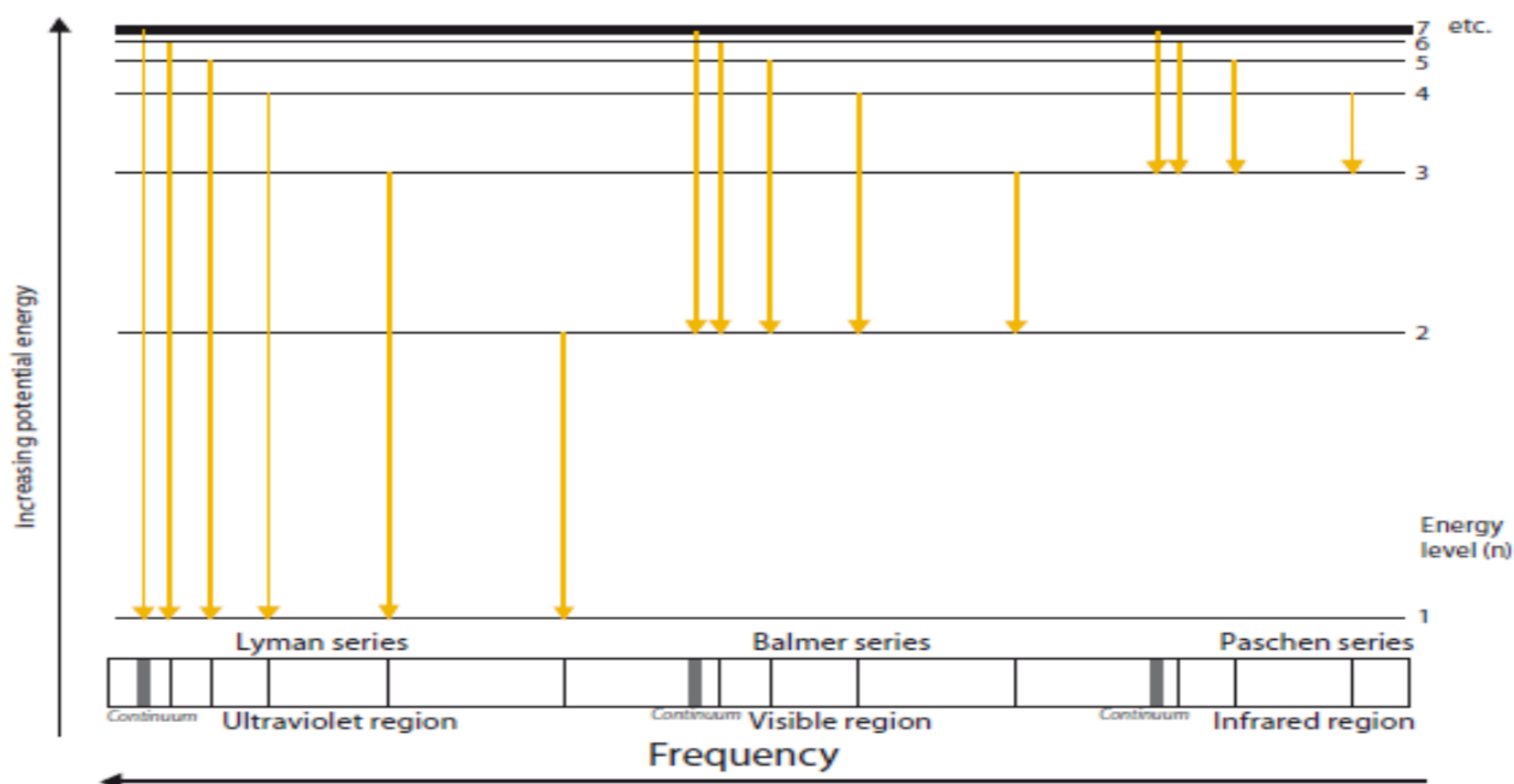
Figure 213 Explanation of the atomic emission spectrum of hydrogen
